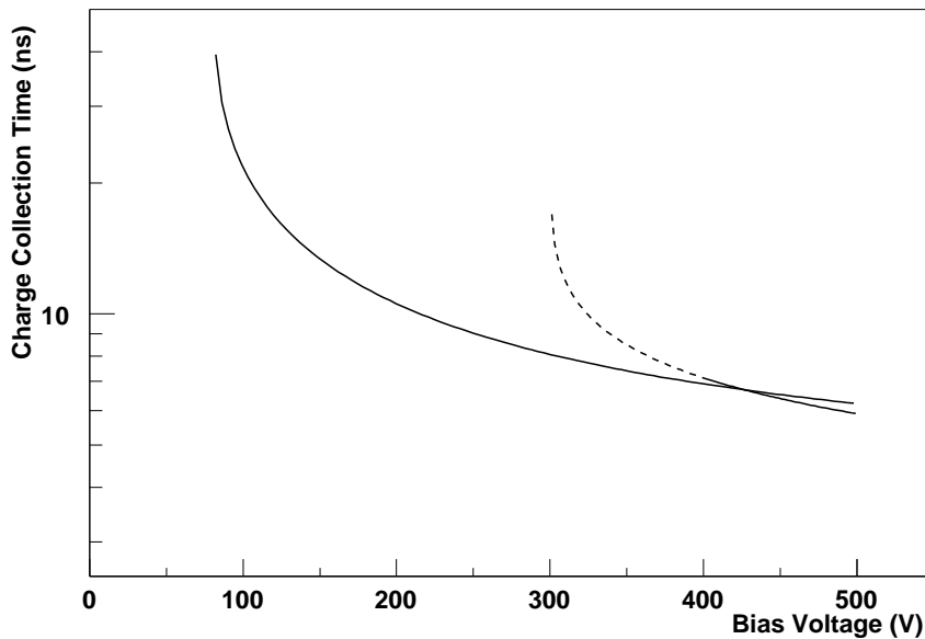
Figure 3.3: Charge collection time as a function of bias voltage. Parameterisation of measurements on a non-irradiated wafer (continuous line) and a wafer irradiated to 2.4 \cdot 10^{14} p/cm^2 (dashed line) in reference [93]
