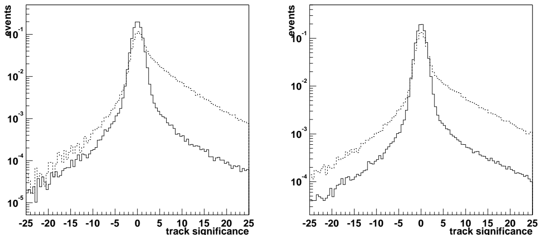
Figure 5.4: Track significance distributions for u (continuous line) and b jets (dashed line). The leftmost figure corresponds to the m_H = 120 GeV sample, the rightmost figure to a 400 GeV Higgs.
